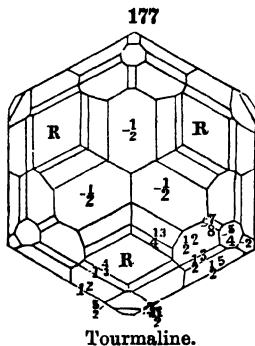
Tourmaline.
